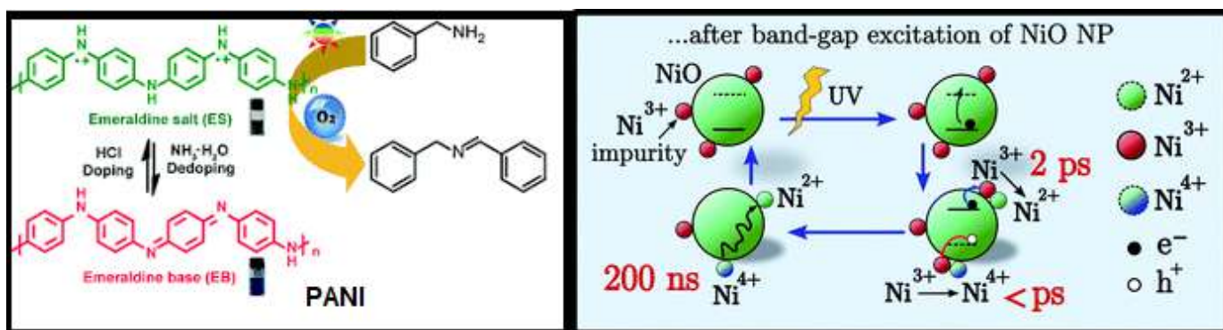
Scheme 2: Schematic presentation of mechanism of UV-radiation in NiO and PANI/NiO nanocomposites
