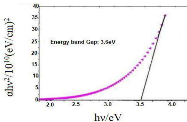
Fig. 2(a): Tauc plot of NiO
